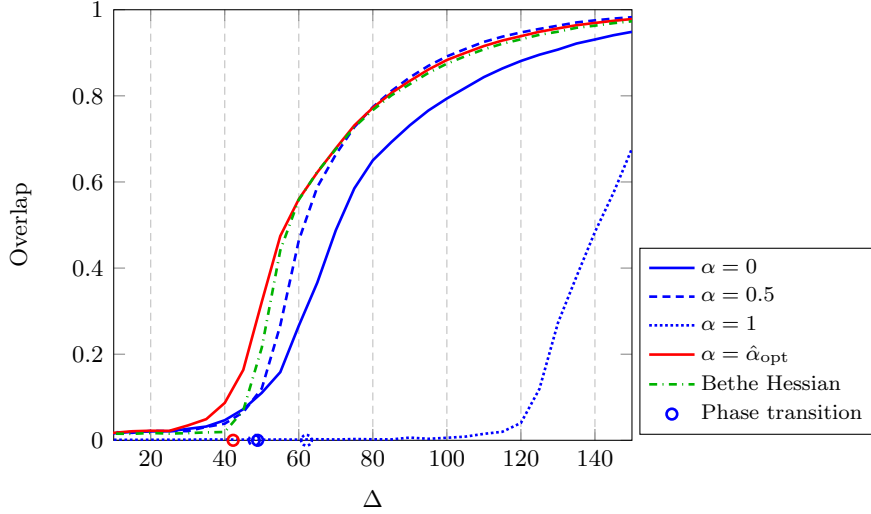
Figure 12: Overlap for n = 3000 , K = 3 , c_i = \frac{1}{3} , \mu a power law with exponent 3 and support [0.05, 0.3] , \mathbf{M} = \Delta \mathbf{I}_3 , for \Delta \in [10, 150] . Here \hat{\alpha}_{\text{opt}} = 0.28 .
