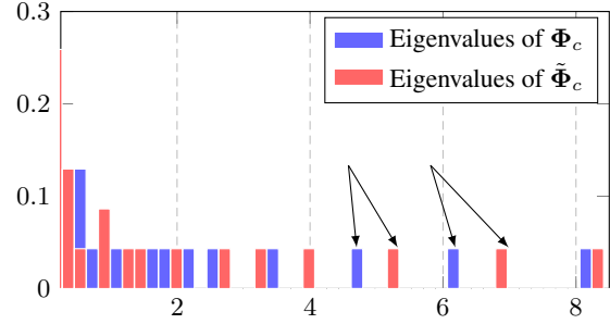
Figure 9. Eigenvalue distribution of \Phi_c and \tilde{\Phi}_c for the epileptic EEG, with the ReLU function, p = 100 , T = 128 and c_1 = c_2 = \frac{1}{2} , with \mathbf{j}_1 = [\mathbf{1}_{T_1}; \mathbf{0}_{T_2}] and \mathbf{j}_2 = [\mathbf{0}_{T_1}; \mathbf{1}_{T_2}] . Expectation estimated by averaging over 500 realizations of \mathbf{W} .
