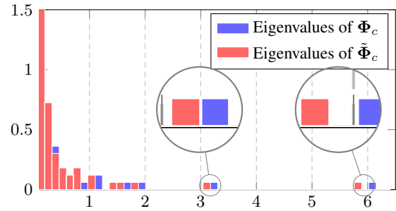
Figure 7. Eigenvalue distribution of \tilde{\Phi}_c and \tilde{\Phi}_c for the MNIST data, with the ReLU function, p = 784 , T = 128 and c_1 = c_2 = \frac{1}{2} , with \mathbf{j}_1 = [\mathbf{1}_{T_1}; \mathbf{0}_{T_2}] and \mathbf{j}_2 = [\mathbf{0}_{T_1}; \mathbf{1}_{T_2}] . Expectation estimated by averaging over 500 realizations of \mathbf{W} .
