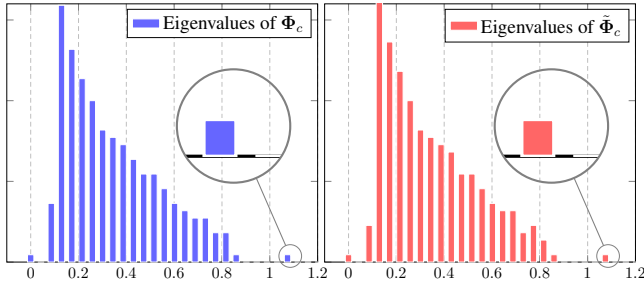
Figure 1. Eigenvalue distribution of \Phi_c and \tilde{\Phi}_c for the ReLU function and Gaussian mixture data with \boldsymbol{\mu}_a = [\mathbf{0}_{a-1}; 3; \mathbf{0}_{p-a}] , \mathbf{C}_a = \left(1 + \frac{2(a-1)}{\sqrt{p}}\right) \mathbf{I}_p , p = 512 , T = 256 and c_1 = c_2 = \frac{1}{2} . Expectation estimated by averaging over 500 realizations of \mathbf{W} .
