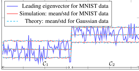
Figure 8. Leading eigenvector of \Phi_c for the MNIST and Gaussian mixture data with a width of \pm 1 standard deviations (generated from 500 trials) in the settings of Figure 7.
