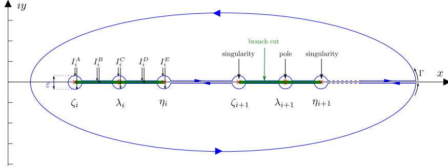
Fig. B.7: Chosen integration contour. The set I_i^B is the disjoint union of the segments [\zeta_i + \varepsilon + 0^+ \iota, \lambda_i - \varepsilon + 0^+ \iota] and [\zeta_i + \varepsilon + 0^- \iota, \lambda_i - \varepsilon + 0^- \iota] . Similarly the set I_i^D is the disjoint union of the segments [\lambda_i + \varepsilon + 0^+ \iota, \eta_i - \varepsilon + 0^+ \iota] and [\lambda_i + \varepsilon + 0^- \iota, \eta_i - \varepsilon + 0^- \iota] . The sets I_i^A , I_i^C and I_i^E are the disjoint unions of semi-circles (in the upper- or lower-half complex plane) of diameters \varepsilon surrounding \zeta_i , \lambda_i and \eta_i respectively.
