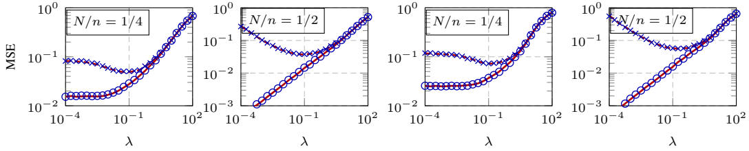
Figure 7: MSEs of RFF regression on Fashion-MNIST ( left two ) and Kannada-MNIST ( right two ) data (class 5 versus 6), as a function of regression parameter \lambda , for p = 784 , n = \hat{n} = 1024 , N = 256 and 512 . Empirical results displayed in blue (circles for training and crosses for test); and the asymptotics from Theorem 2 and 3 displayed in red (solid lines for training and dashed for test). Results obtained by averaging over 30 runs.
