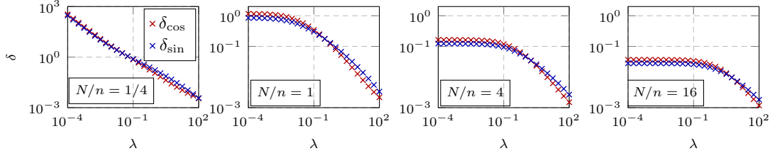
Figure 2: Behavior of (\delta_{\cos}, \delta_{\sin}) in (9) on MNIST data (class 3 versus 7), as a function of the regularization parameter \lambda , for p = 784 , n = 1000 , N = 250, 1000, 4000, 16000 .
