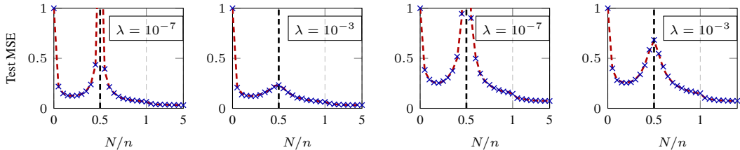
Figure 9: Empirical ( blue crosses) and theoretical ( red dashed lines) test error of RFF regression, as a function of the ratio N/n , on Fashion-MNIST ( left two ) and Kannada-MNIST ( right two ) data (class 8 versus 9), for p = 784 , n = 500 , \lambda = 10^{-7} and 10^{-3} . The black dashed line is the interpolation threshold 2N = n . Results obtained by averaging over 30 runs.
