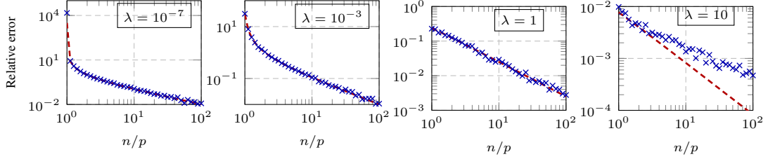
Figure 6: Relative errors of quadratic form approximation |\mathbf{a}^\top(\hat{\mathbf{C}}+\lambda\mathbf{I})^{-1}\mathbf{a}-\mathbf{a}^\top(\mathbf{C}+\lambda\mathbf{I})^{-1}\mathbf{a}|/\mathbf{a}^\top(\mathbf{C}+\lambda\mathbf{I})^{-1}\mathbf{a} , as a function of the ratio n/p , for p = 500 , \lambda = 10^{-7}, 10^{-3}, 1, 10 , \mathbf{C} = \mathbf{I}_p and \mathbf{a} = \mathbf{1}_p/\sqrt{p} . Empirical results displayed in blue crosses and large n, p predictions from (11) in red dashed lines. Results obtained by averaging over 10 runs.
