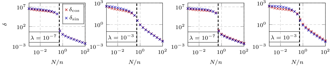
Figure 8: Behavior of (\delta_{\cos}, \delta_{\sin}) in (9), on Fashion-MNIST ( left two ) and Kannada-MNIST ( right two ) data (class 8 versus 9), for p = 784 , n = 1000 , \lambda = 10^{-7} and 10^{-3} . The black dashed line is the interpolation threshold 2N = n .
