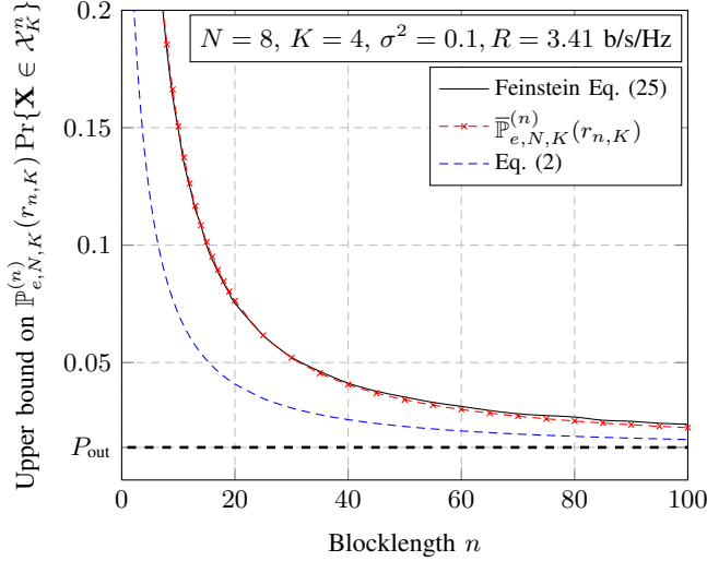
Fig. 2. Upper bounds on the (discounted) error probability \mathbb{P}_{e,N,K}^{(n)}(r_{n,K}) for N = 8, K = 4, \sigma^2 = 0.1, r_{n,K} = 0.85 \times \mathbb{E}[C_{N,K}(\sigma^2)] = 3.41 b/s/Hz, as a function of n , where P_{\text{out}} = \Pr\{C_{N,K}(\sigma^2) < r_{n,K}\} = 1.4\% denotes the outage probability.
